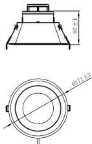
Downlight 28W
