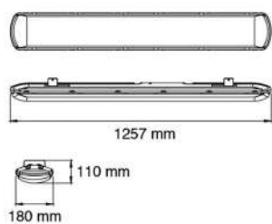
Artic 75W 120°
