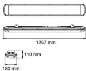
Artic 27W 120°
