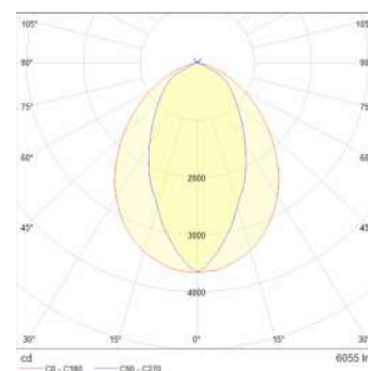
Artic 75W 40*110°
